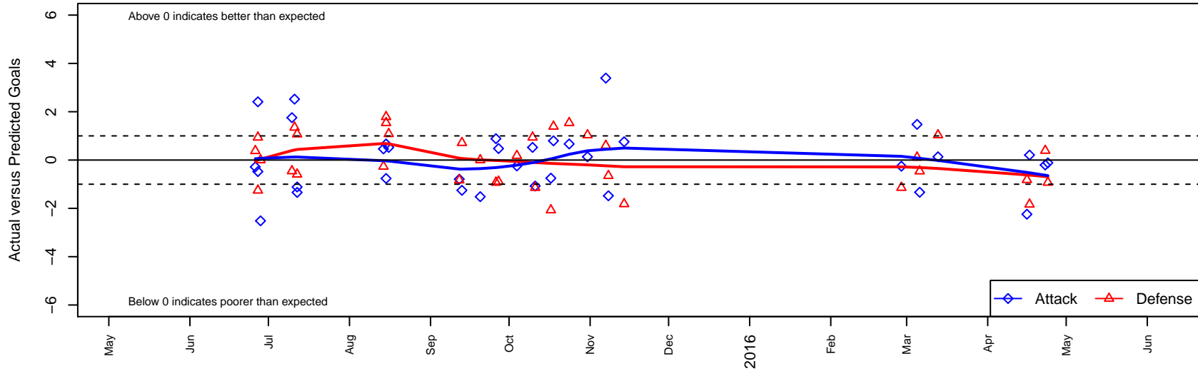
Washington Timbers Forest B02 Dots are actual minus expected GF (blue circles) and GA (red triangles). Blue line is smoothed change in attack strength. Red is smoothed change in defense strength.
